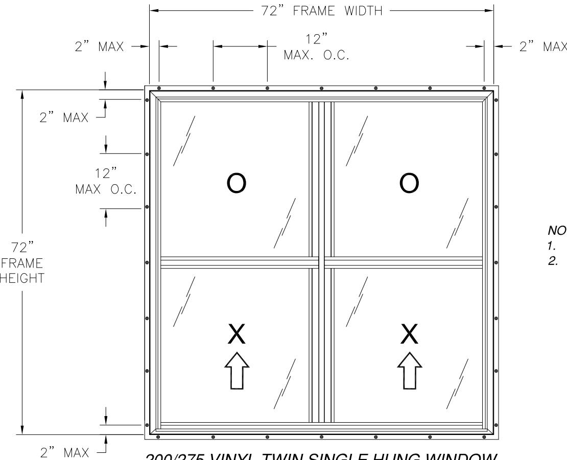
200/275 VINYL TWIN SINGLE HUNG WINDOW EXTERIOR VIEW FIN INSTALLATION
