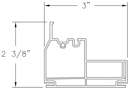
HEAD (9201) EXTRUDED RIGID PVC
