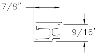
LOCK RAIL/STILE REINFORCEMENT (10712) ALUMINUM 6005-T5
