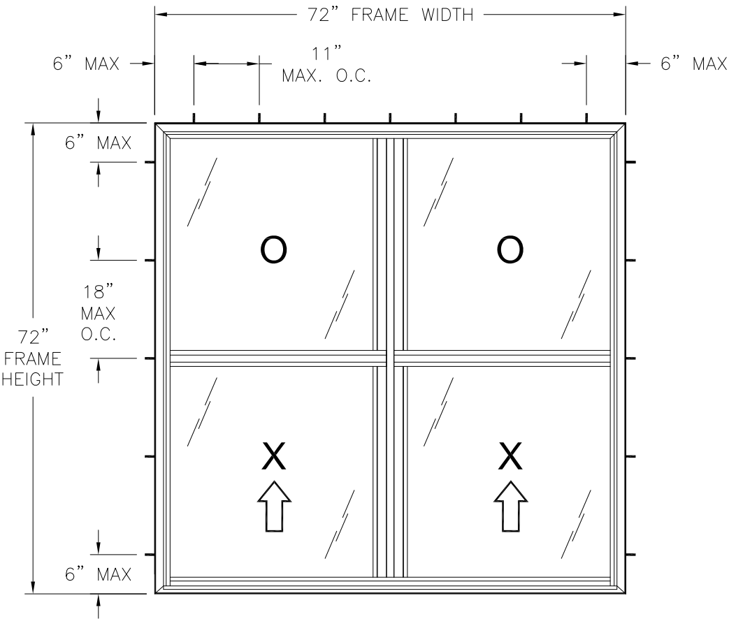
200/275 VINYL TWIN SINGLE HUNG WINDOW EXTERIOR VIEW FRAME INSTALLATION
